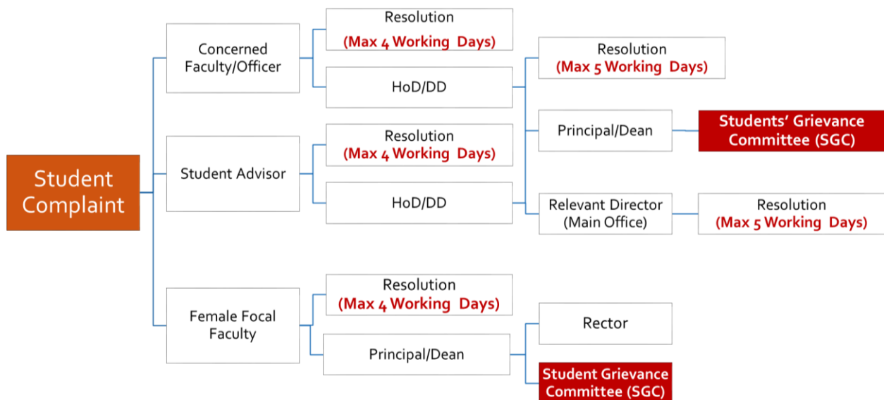
Figure 1: Complaint Process
